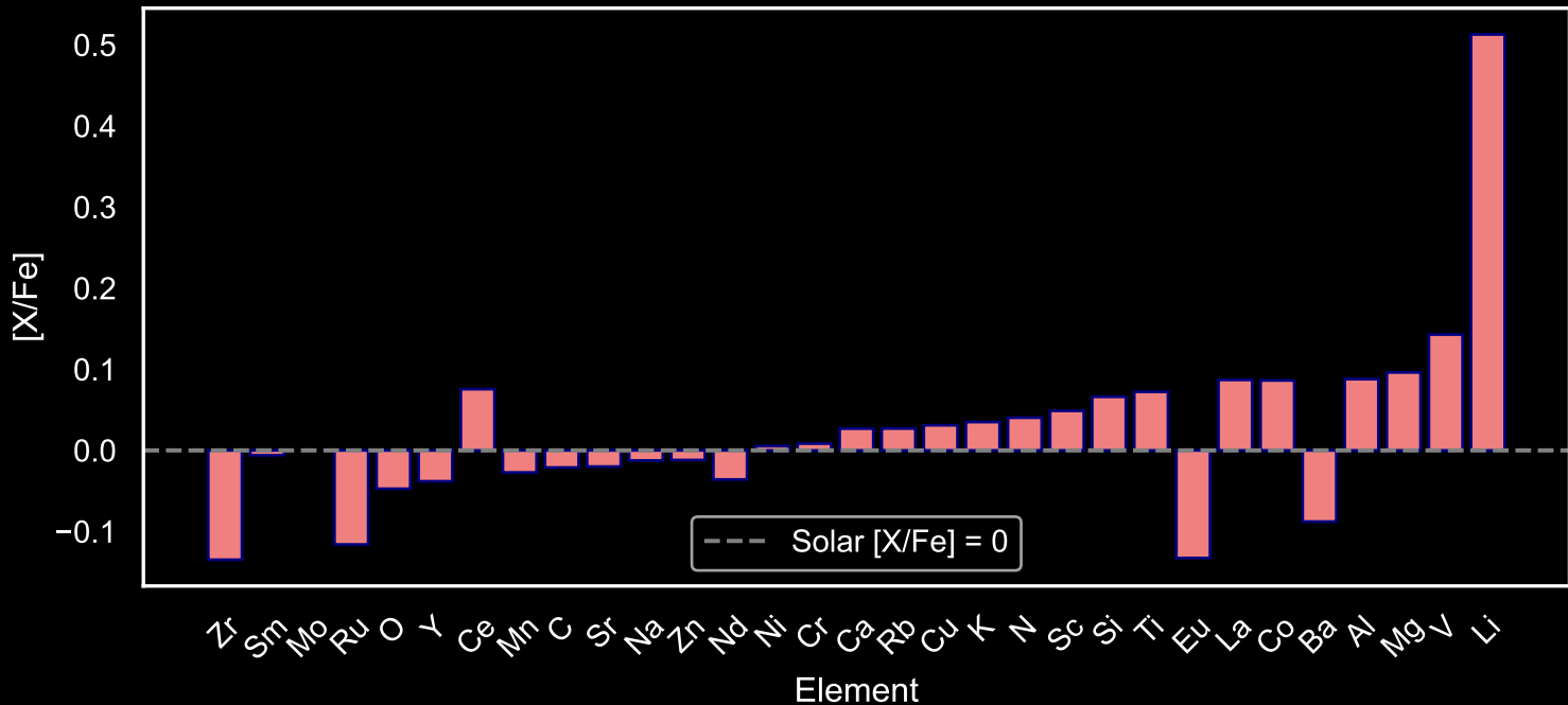
Abundance Pattern for GALAH Main Sequence Stars: Star Field [35] (N=153)
