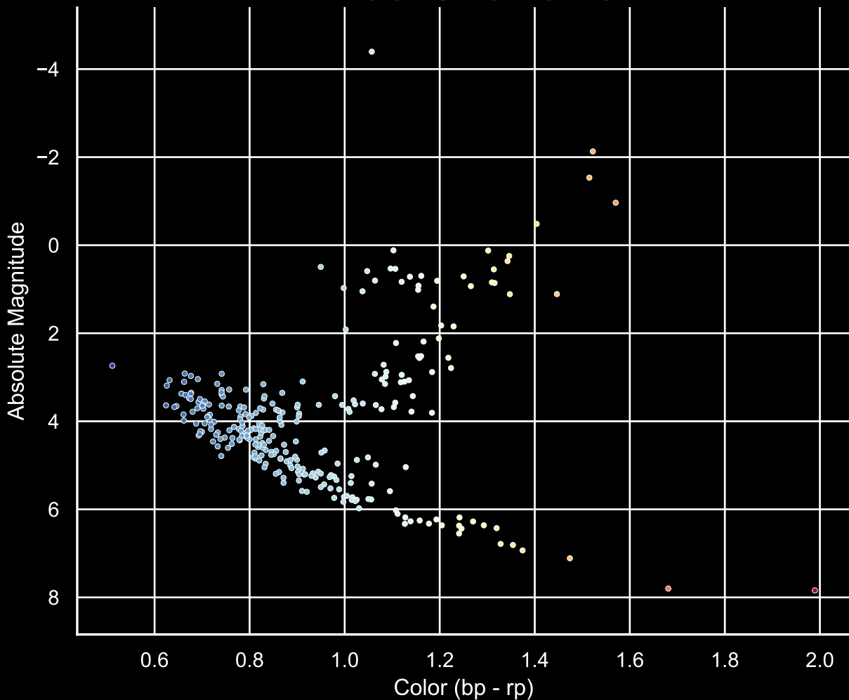
GALAH Hertzsprung-Russel Diagram Field [35] Ra [334.0] Dec [-63.77]
