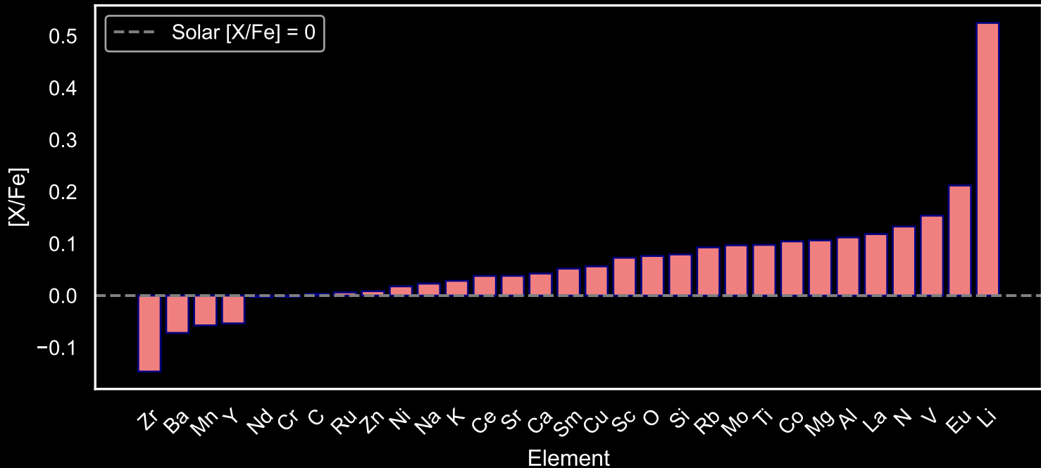
Abundance Pattern for GALAH Star Field [35] (N=286)
