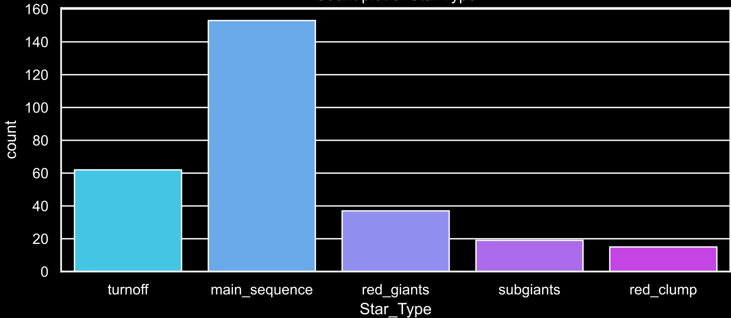
Field [35] Count plot of Star Type
