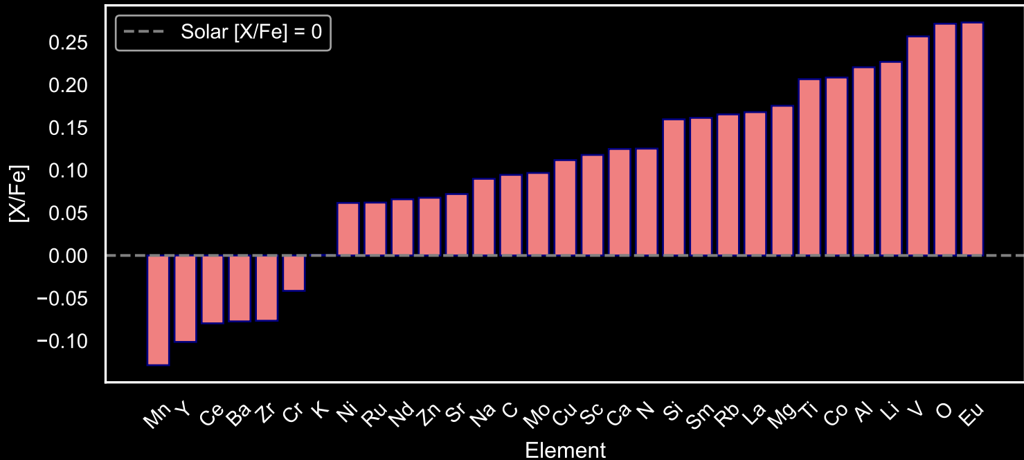
Abundance Pattern for GALAH Red Giants: Star Field [35] (N=52)
